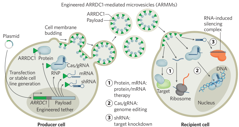
Fig. 1 | Schematic of how engineered ARMMs are produced to enable delivery of therapeutic payloads.
